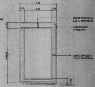
SECTION OF RCBC SCALE: 1:20 M
